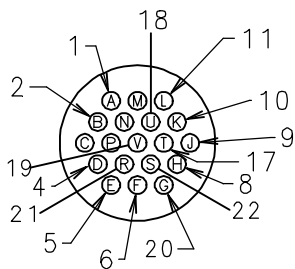
19 pole plug
